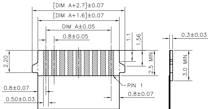
RECOMMENDED FPC/FFC DIMENSIONS GENERAL TOLERANCE ±0.05
